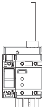
INDICATE OFF / SINGLE COLOR ROCKER ACTUATOR
