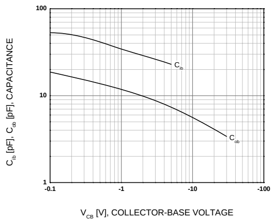
Figure 3. Capacitance
