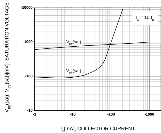
Figure 2. Saturation Voltage
