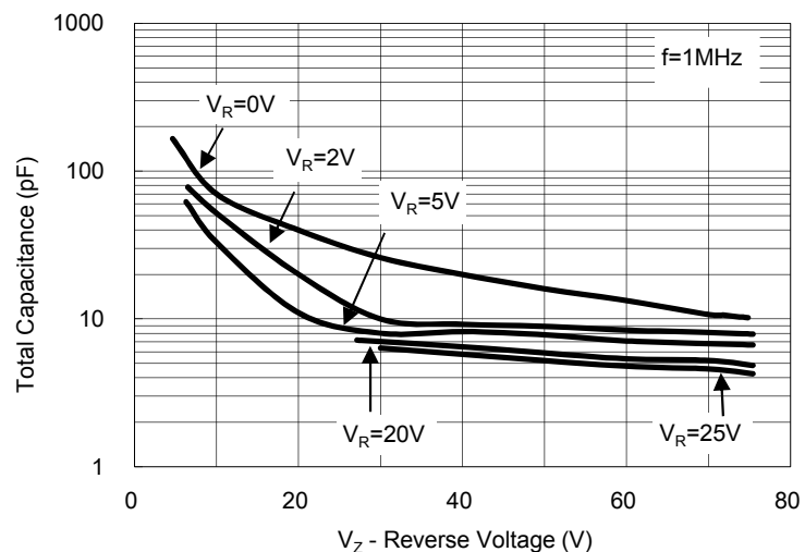
Fig. 2 Total Capacitance
