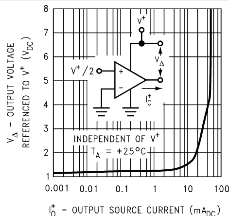
Figure 6-10. Output Characteristics Current Sourcing
