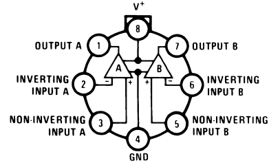
Figure 5-2. LMC Package 8-Pin TO-99 Top View
