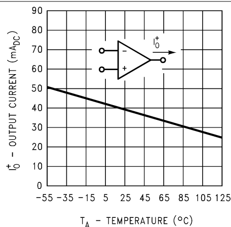
Figure 6-12. Current Limiting
