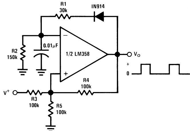
Figure 8-12. Pulse Generator
