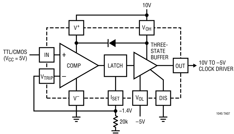
TTL/CMOS ( V_{CC} = 5V ) to 10V/ -5V Clock Driver
