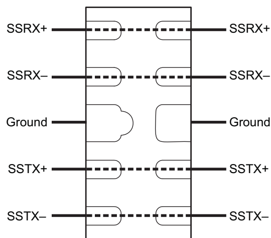
Figure 4. Flow Through Layout for USB 3.0
