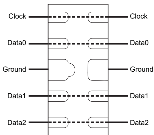
Figure 3. Flow Through Layout for HDMI
