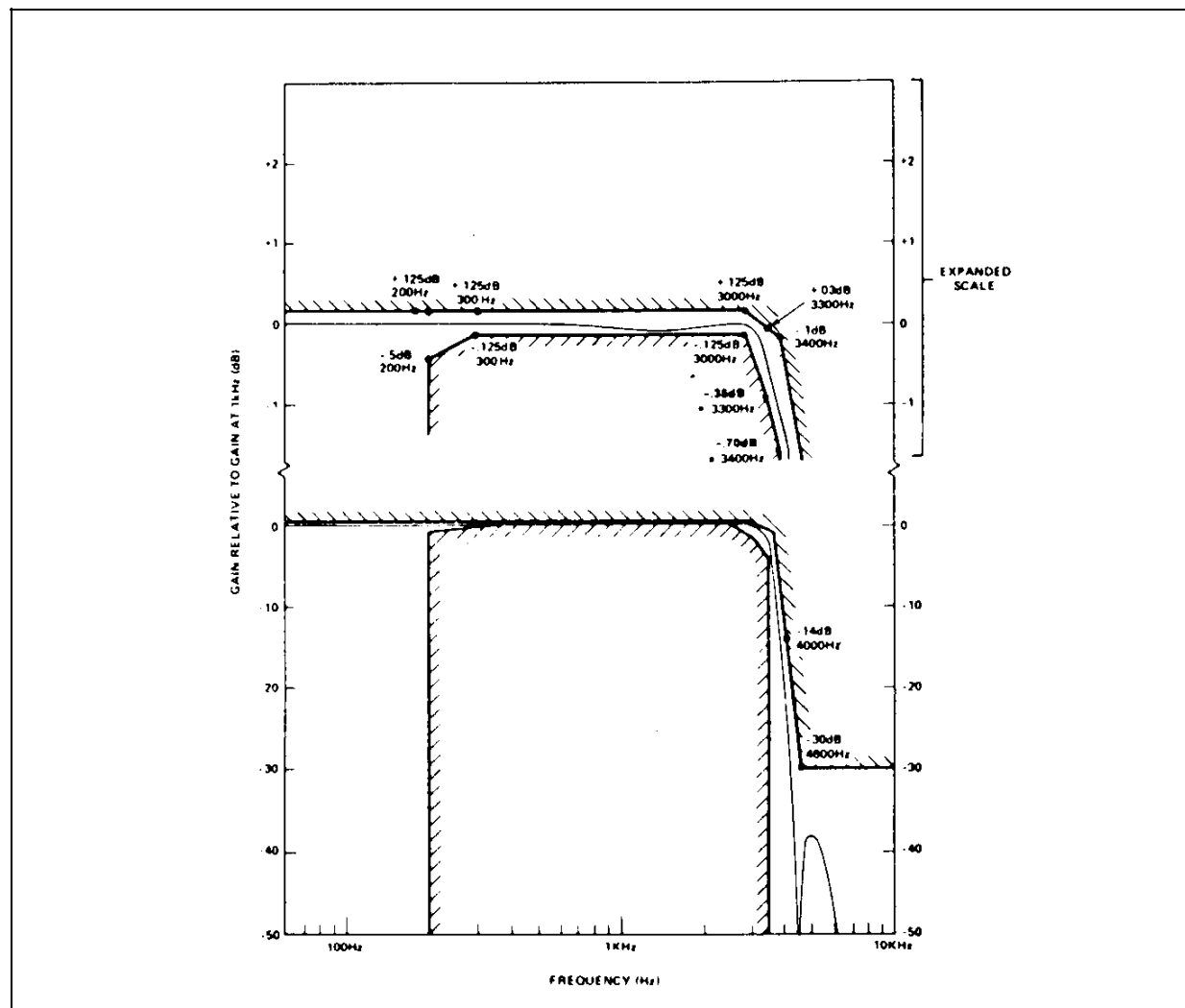
Figure 6: Receive Filter
