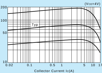
h FE -I C Characteristics (Typical)
