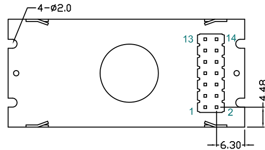
DOTS DETAIL
