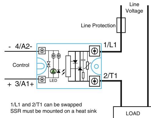
Figure 1c — SHXXRXX relays
