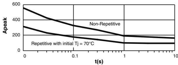
Figure 3c — 50A output current
