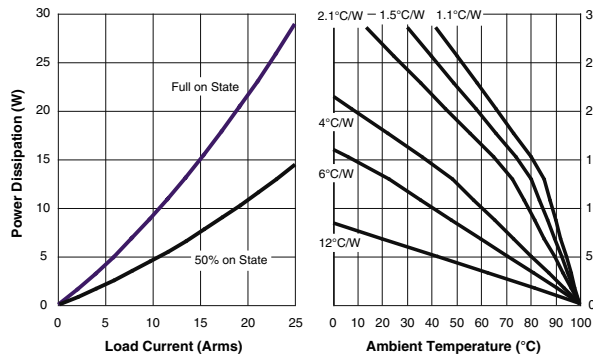
Figure 4a — 25A output power
