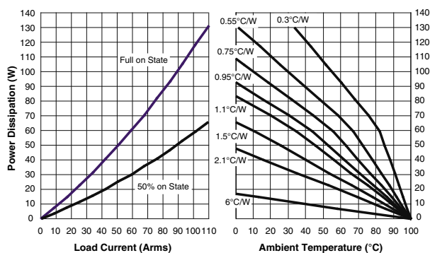
Figure 4e — 95A output power
