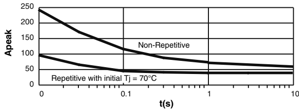
Figure 3a — 25A output current
