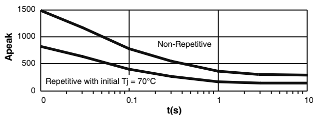
Figure 3e — 95A output current
