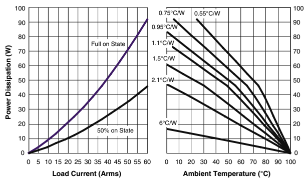
Figure 4c — 50A output power
