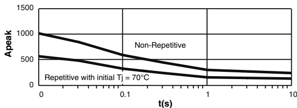
Figure 3d — 75A output current
