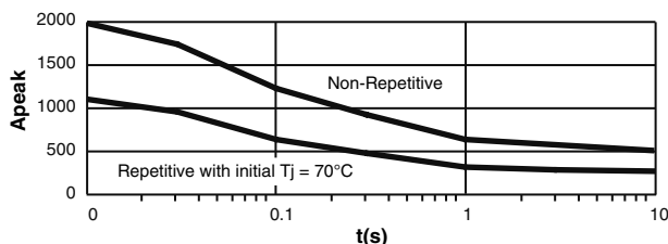
Figure 3f — 125A output current
