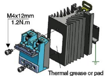
Thermal grease or pad
