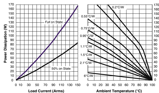
Figure 4f — 125A output power
