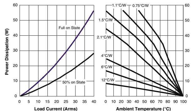
Figure 4b — 35A output power
