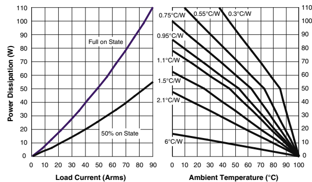
Figure 4d — 75A output power
