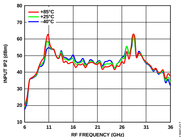
Figure 17. Input IP2 vs. RF Frequency over Various Temperatures, P_{LO} = 15 dBm
