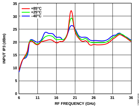
Figure 16. Input IP3 vs. RF Frequency over Various Temperatures, P_{LO} = 15 dBm
