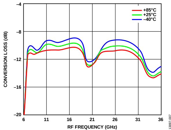
Figure 15. Conversion Loss vs. RF Frequency over Various Temperatures, P_{LO} = 15 dBm
