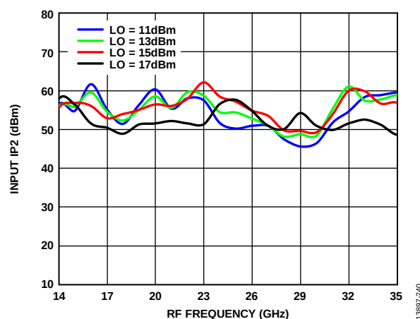
Figure 40. Input IP2 vs. RF Frequency over Various LO Drives
