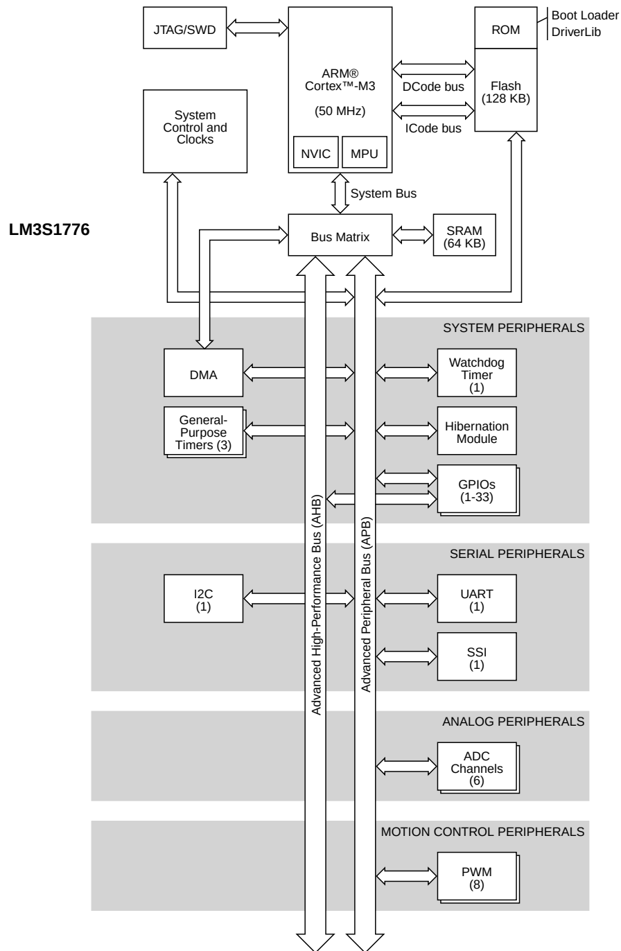
Figure 1-1. Stellaris® LM3S1776 Microcontroller High-Level Block Diagram
