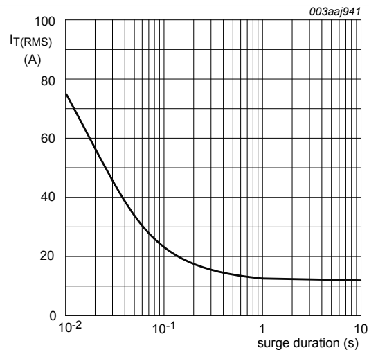
Fig. 2. RMS on-state current as a function of surge duration; maximum values f = 50\text{ Hz} ; T_h = 56\text{ °C}
