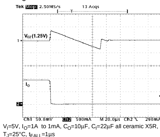
Figure 23 : Short Circuit Removal Response
