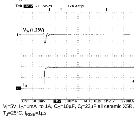
Figure 21 : Change of V_O with Step Load Change
