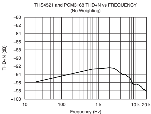
Figure 81. THS4521 and PCM3168: Thd+N Versus Frequency With No Weighting
