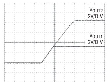
FIGURE 13 CIRCUIT 38271 G09
