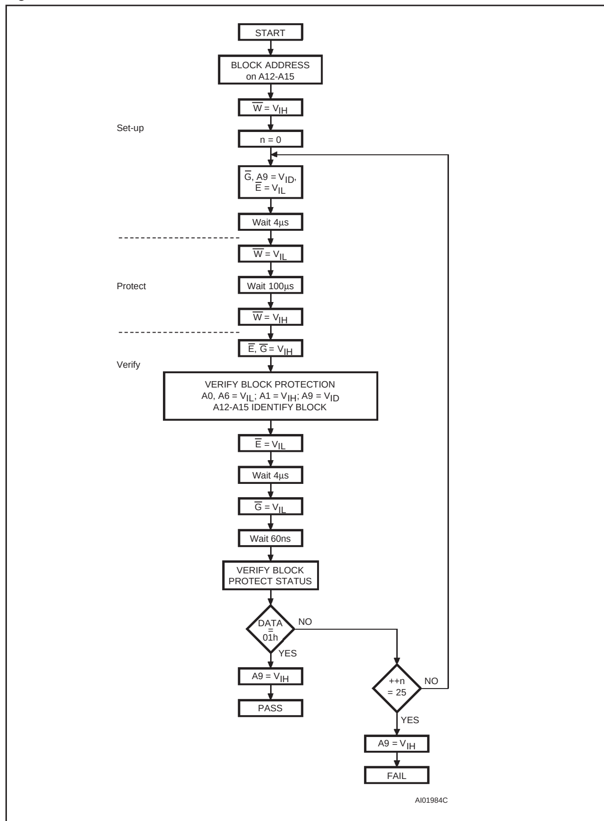
Figure 14. BlockProtection Flowchart
