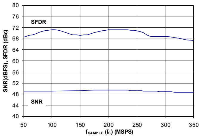
FIGURE 7. SNR AND SFDR vs f_{\text{SAMPLE}}
