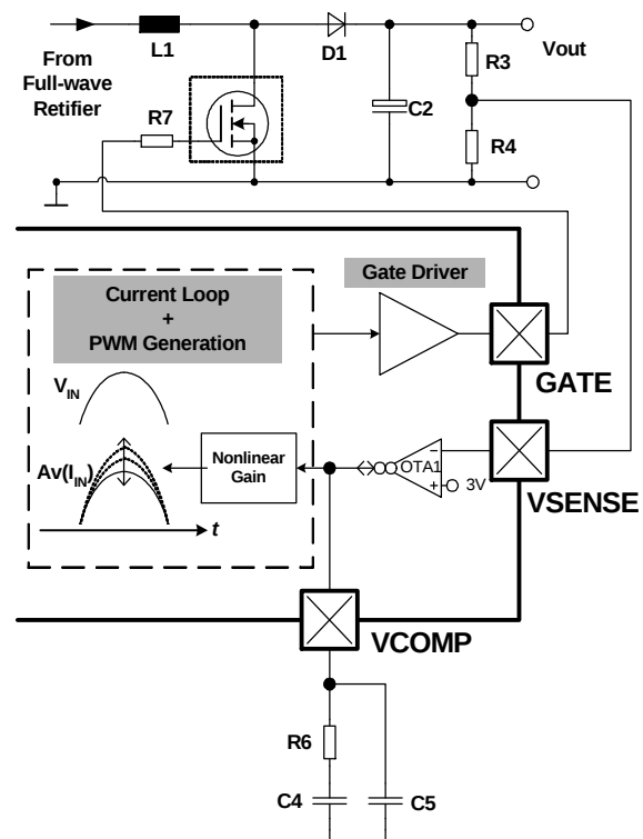
Figure 15 Voltage Loop
