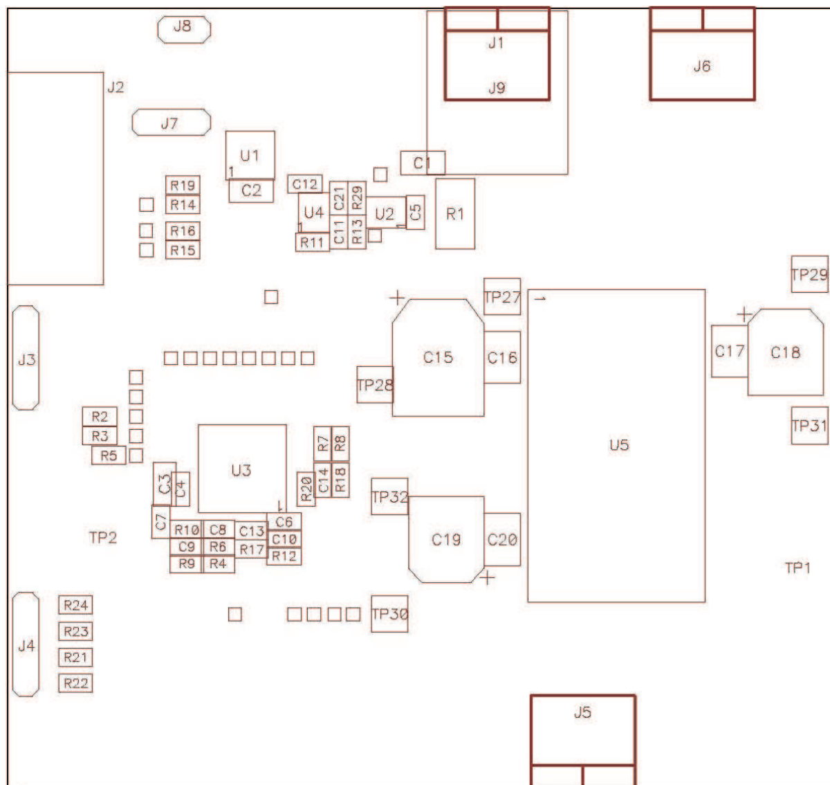
Figure 13. Top Layer Assembly Drawing (top view)
