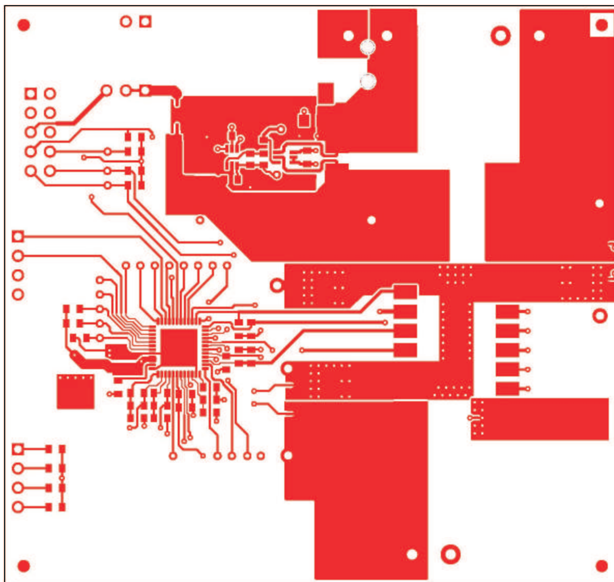
Figure 14. Top Copper (top view)
