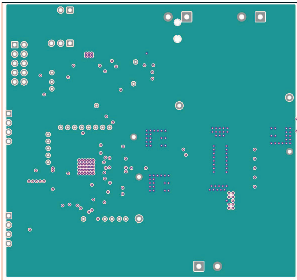
Figure 15. Internal Layer 1 (top view)
