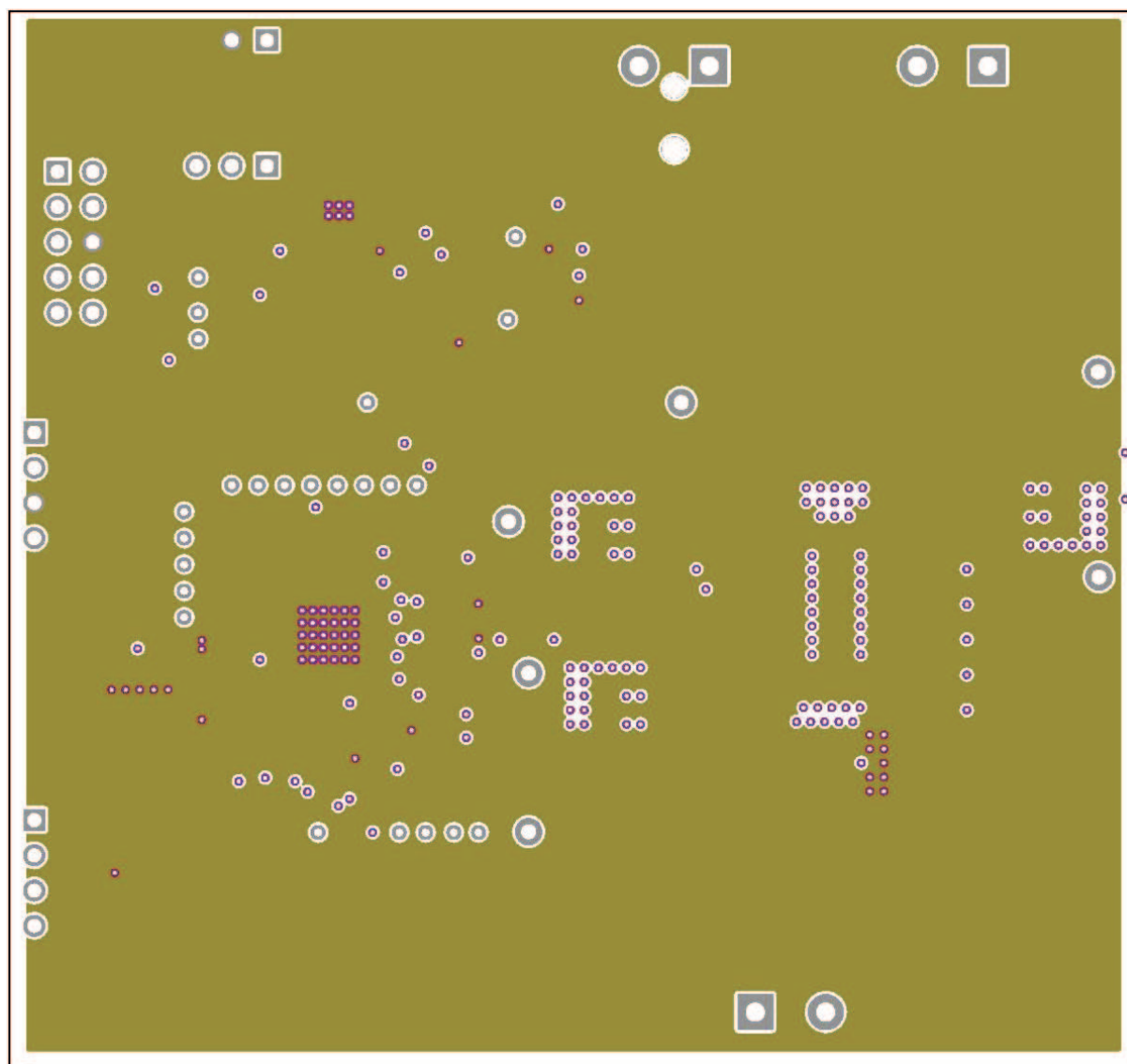
Figure 16. Internal Layer 2 (top view)
