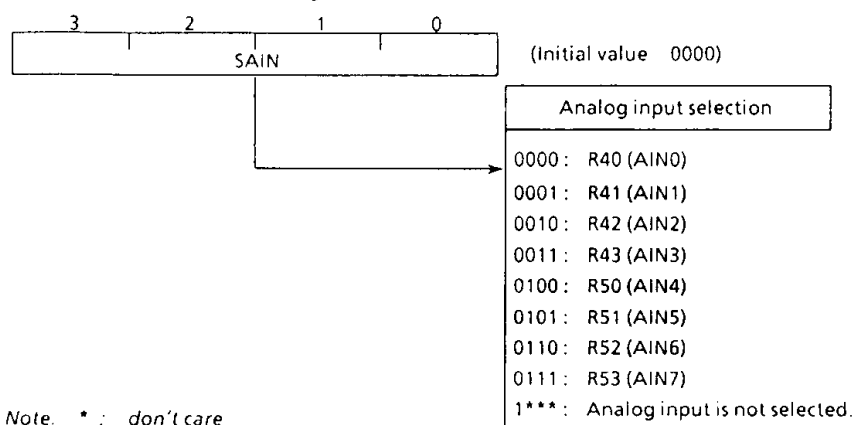
Figure 3-22. Analog input selector
