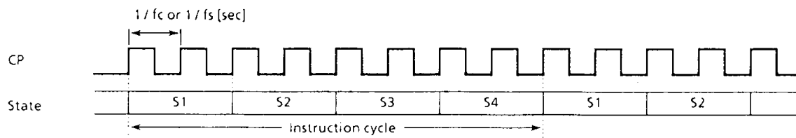
Figure 2-20. Instruction Cycle
