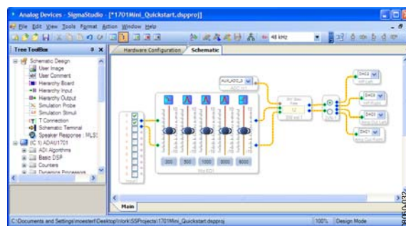
Figure 4. Schematic Tab, Full Design
