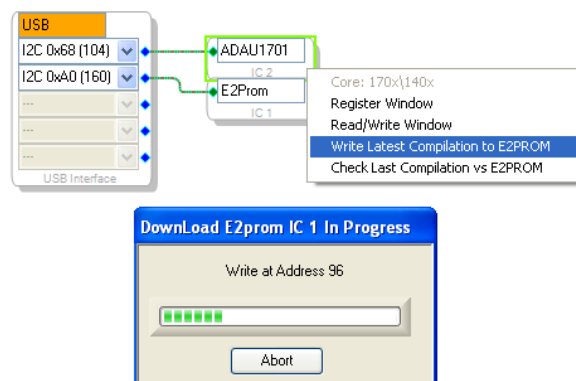
Figure 9. SigmaStudio Downloading to Self-Boot EEPROM
