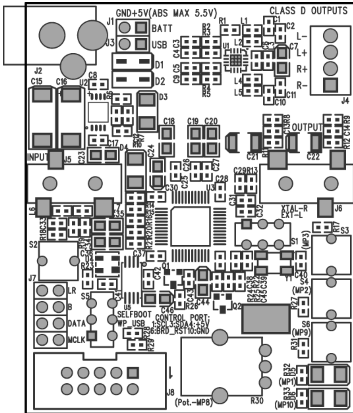
Figure 15. Board Layout
