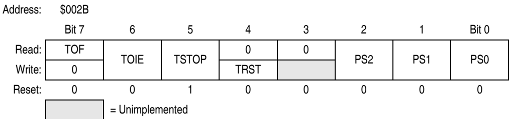
Figure 18-5. TIM2 Status and Control Register (T2SC)
