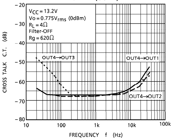
CT - f(OUT-4)
