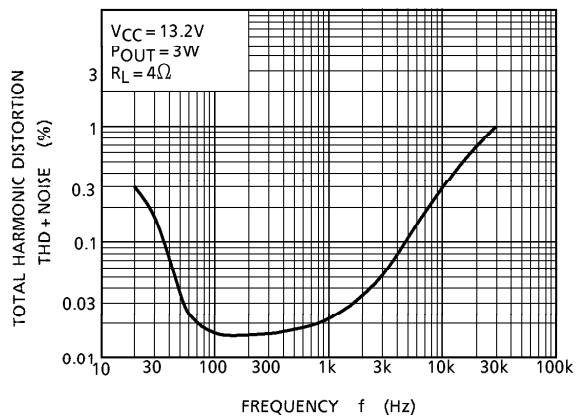
THD - f
