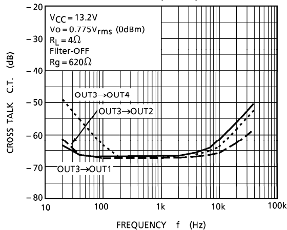
CT - f(OUT-3)
