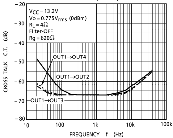
CT - f(OUT-1)
