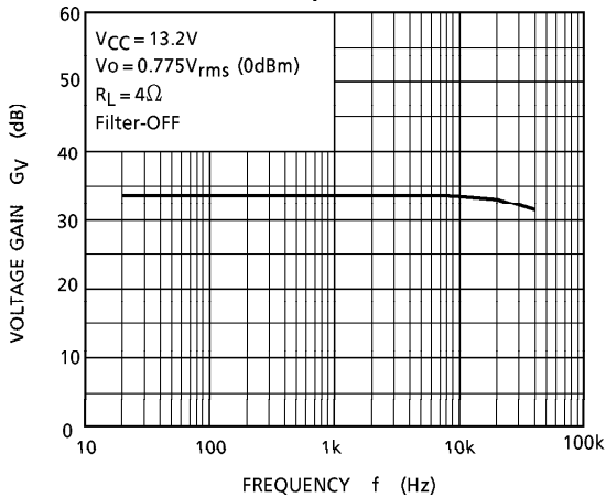
G_V - f
