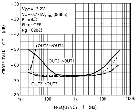
CT - f(OUT-2)
