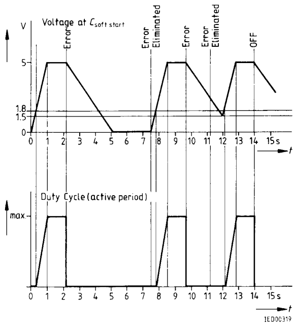
Soft Start/Error/ON-OFF
