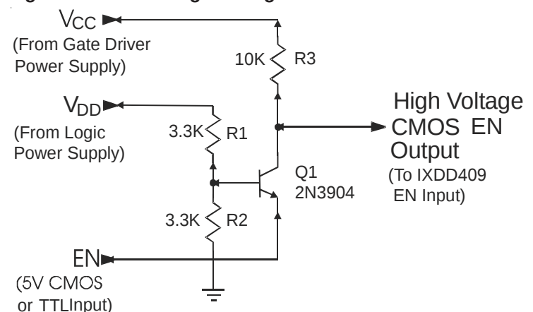
Figure 27 - TTL to High Voltage CMOS Level Translator
