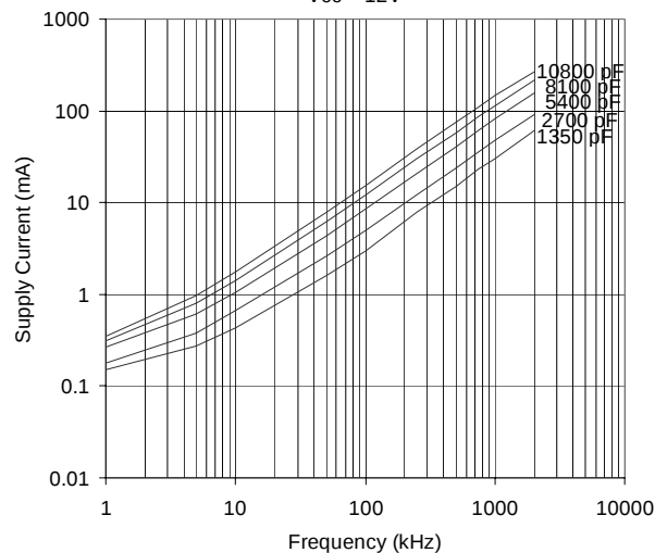
Fig. 12 Supply Current vs. Frequency V CC = 12V
