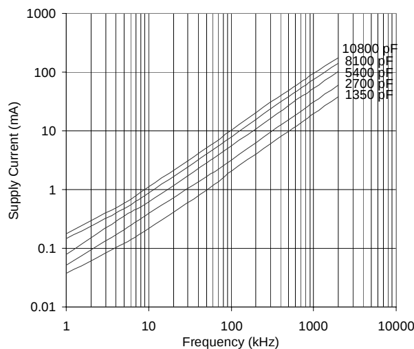
Fig. 14 Supply Current vs. Frequency V CC = 8V
