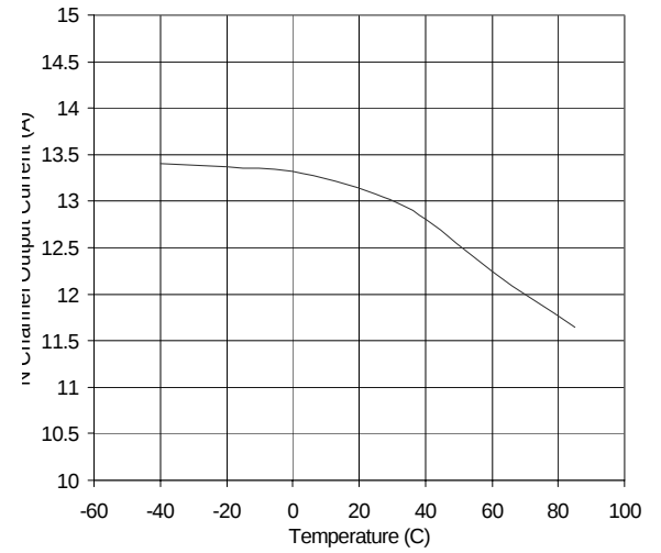
Fig. 22 N Channel Peak Output Current vs. Temperature V_{CC} = 18V CL = 10\text{ nF}
