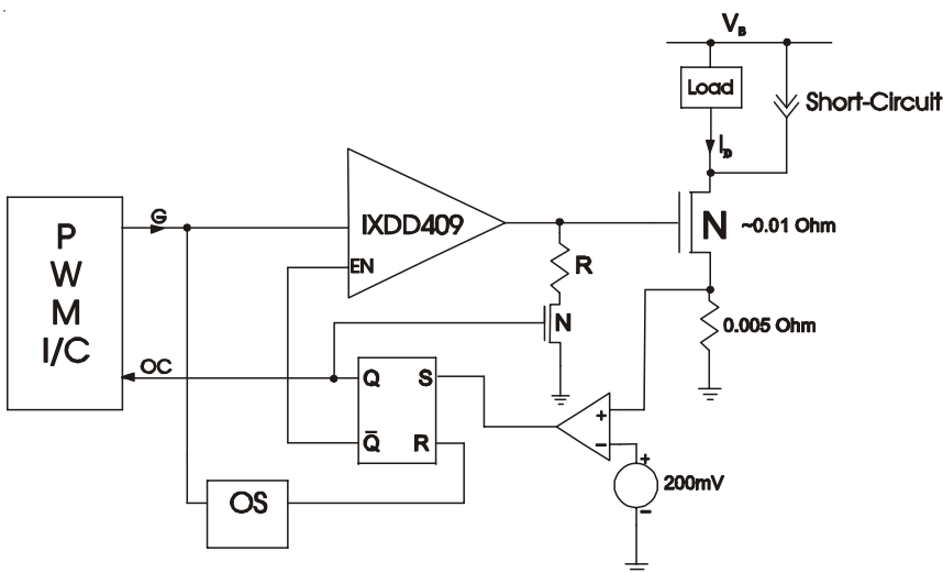
Figure 25 - Typical Application Short Circuit di/dt Limit
