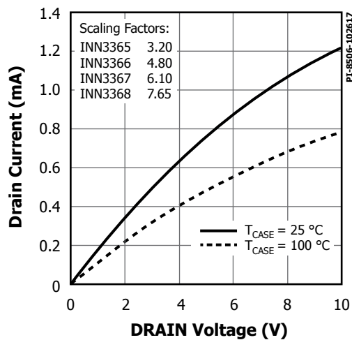
Figure 40. Output Characteristics.
