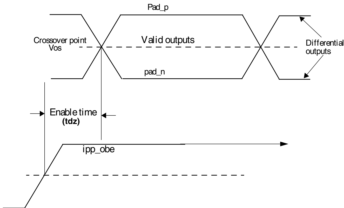
Figure 6. Enable time
