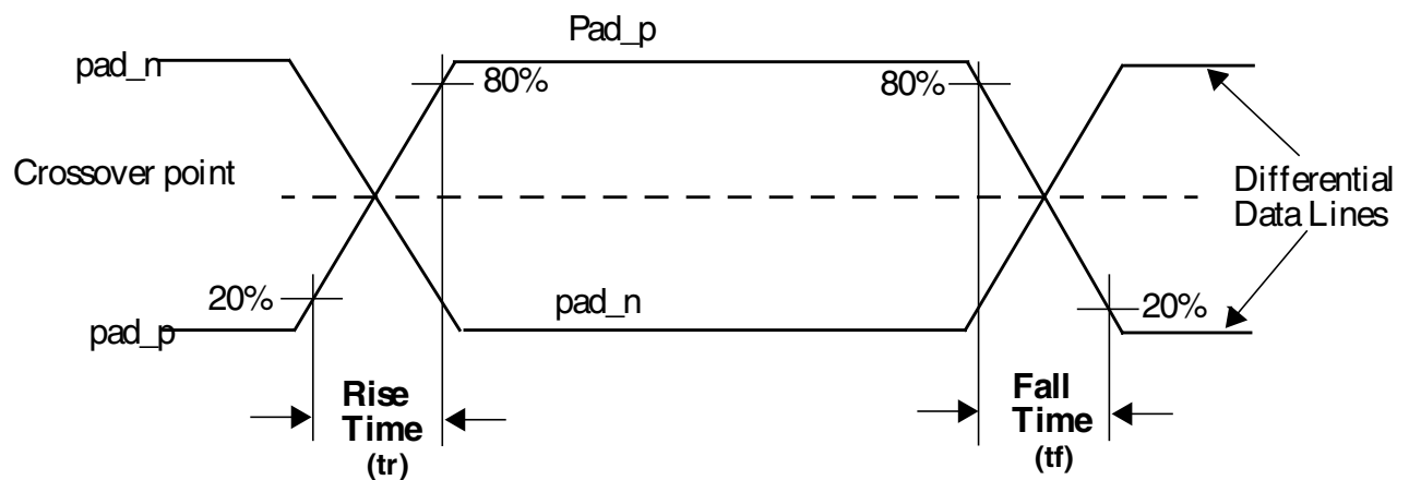
Figure 5. Rise/Fall transition
