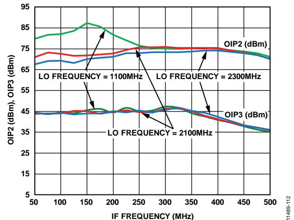
Figure 12. OIP2/OIP3 vs. IF Frequency; RF Sweep with Fixed LO; IF and RF Roll-Off; Measured on 1 V p-p on Each Tone at DGA Output
