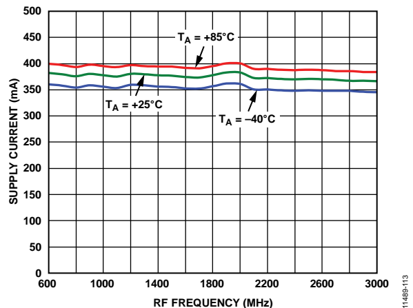
Figure 13. Supply Current vs. RF Frequency
