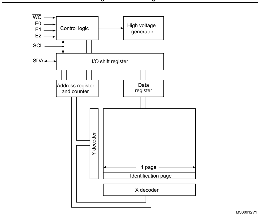
Figure 8. Block diagram
