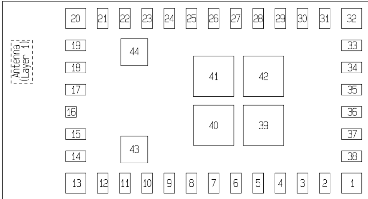
Figure 3 Module Bottom View
