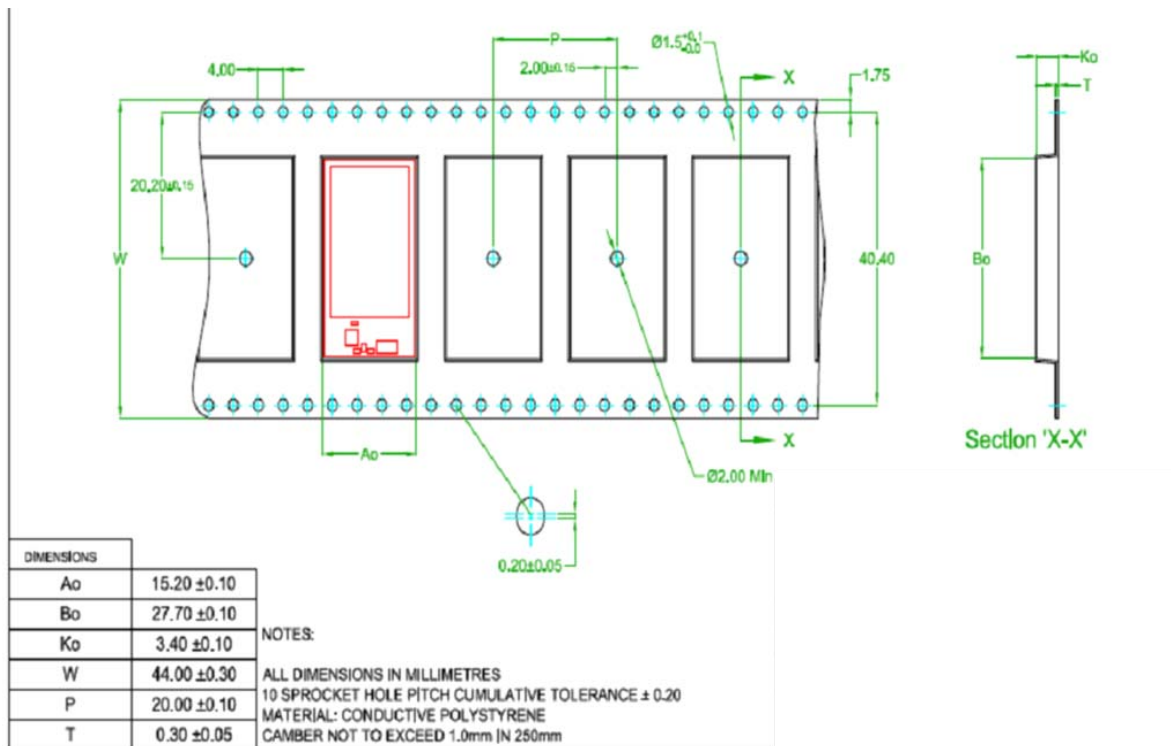
Figure 14 Tape Dimensions
