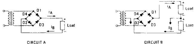
FIGURE 13 – BASIC CIRCUIT USES FOR BRIDGE RECTIFIERS
