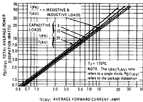
FIGURE 11 – POWER DISSIPATION
