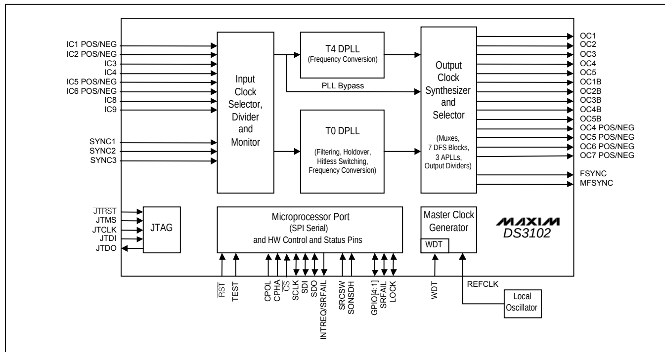
Figure 3-1. Block Diagram
