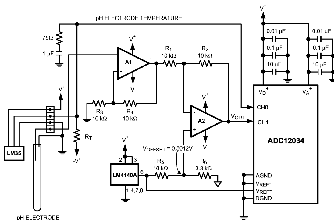
FIGURE 12. pH Measurement Circuit
