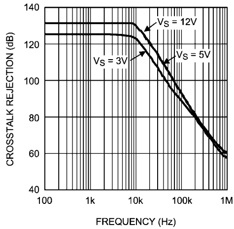
Crosstalk Rejection Ratio vs. Frequency (LMP7702/LMP7704)
