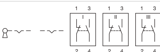
Wiring diagram 113
