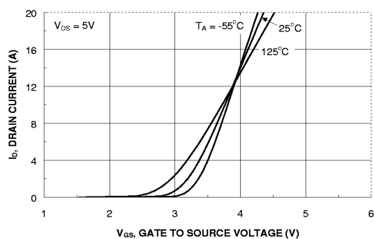
Figure 5. Transfer Characteristics.
