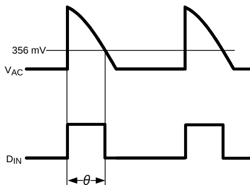
Figure 27. Phase Angle Demodulation
