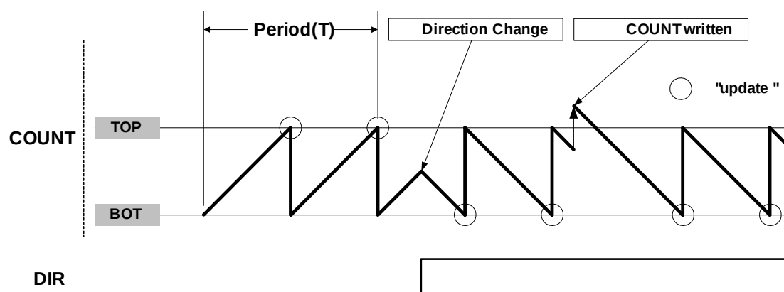
Figure 27-3. Counter Operation
