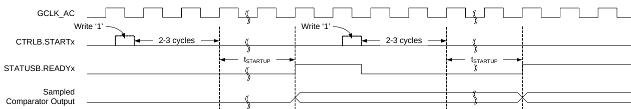
Figure 29-3. Single-Shot Example
