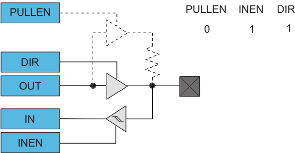
Figure 21-7. I/O Configuration - Totem-Pole Output with Enabled Input
