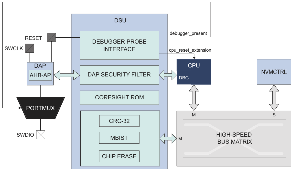
Figure 12-1. DSU Block Diagram
