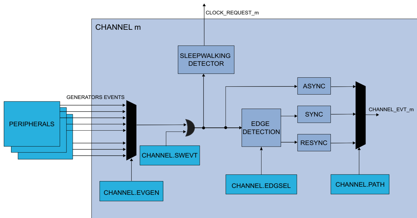
Figure 22-3. Channel
