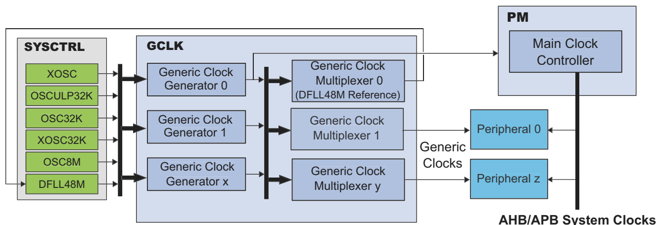
Figure 13-1. Clock distribution
