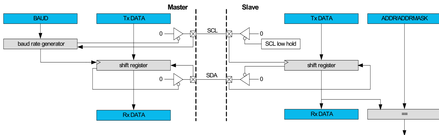
Figure 26-1. I 2 C Single-Master Single-Slave Interconnection
