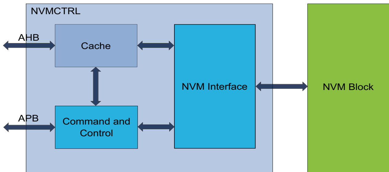
Figure 20-1. Block Diagram
