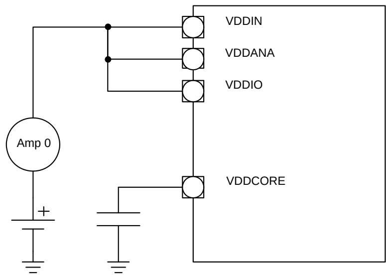
Figure 32-1. Measurement Schematic
