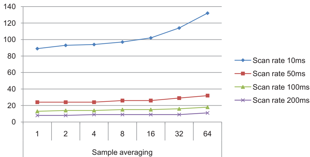
Figure 32-5. Power consumption [ \mu A]. 1 sensor, noise countermeasures disabled, f=48MHz, Vcc=3.3V
