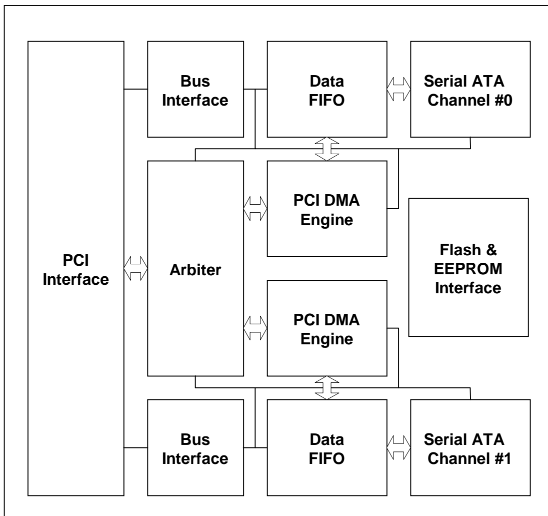
Figure 11. Sil3512 Block Diagram
