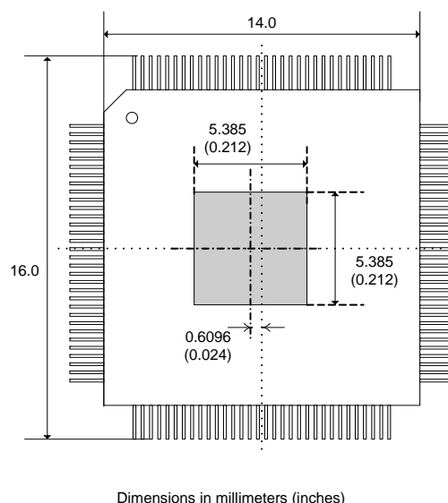
Figure 7. Top View of Enhanced 128-pin TQFP Package
