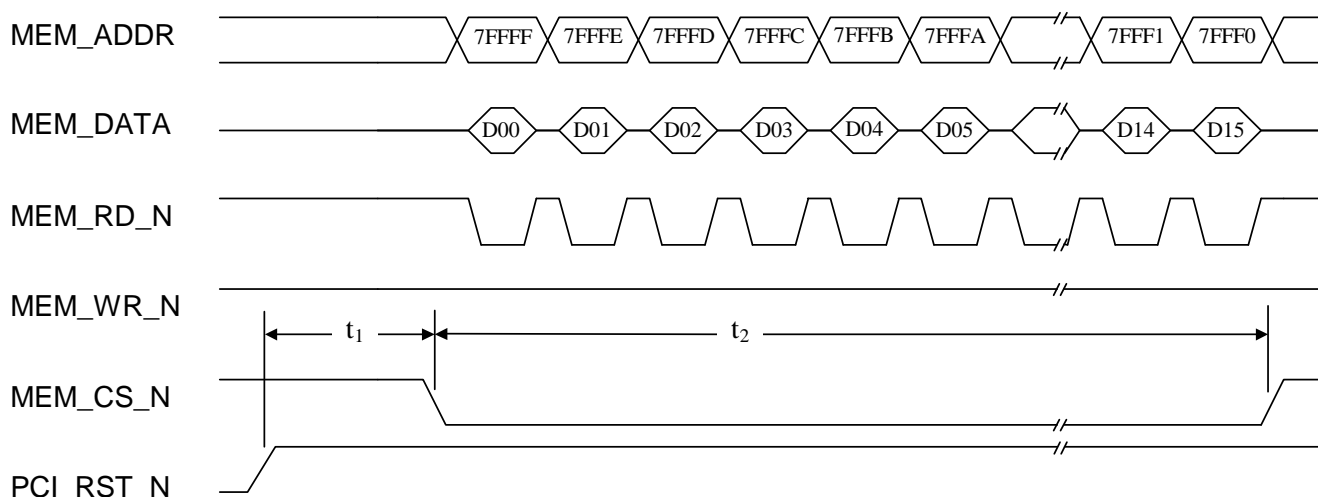
Figure 12. Auto-Initialization from Flash Timing
