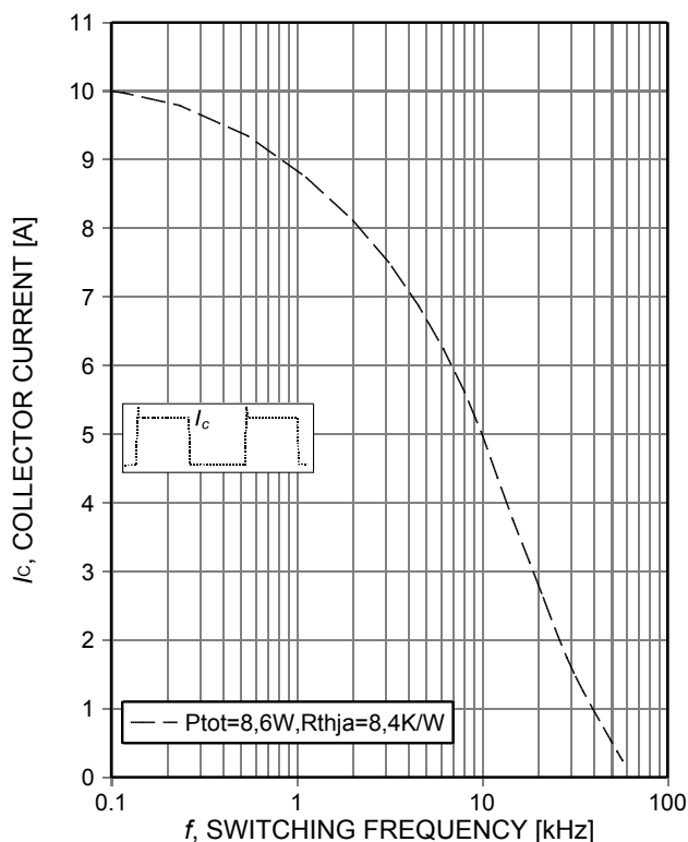
Figure 1. Collector current as a function of switching frequency ( T_{vj} \leq 175^\circ C , T_a = 55^\circ C , D = 0.5 , V_{CE} = 400V , V_{GE} = 15/0V , r_G = 23\Omega , PCB mounting with thermal vias and heatsink, see Appnote: www.infineon.com/igbt )
