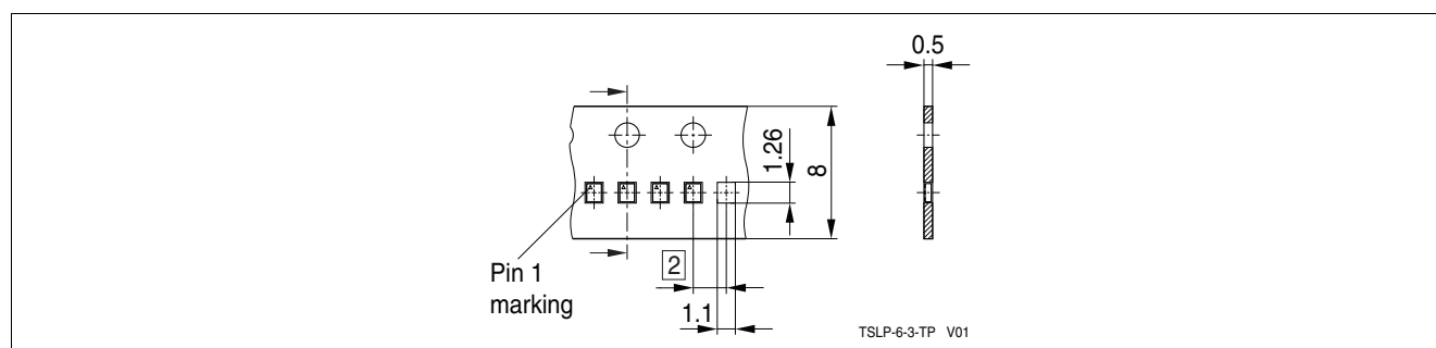
Figure 9 Tape & Reel Dimensions (Ø reel 180 mm, pieces/reel 15000)
