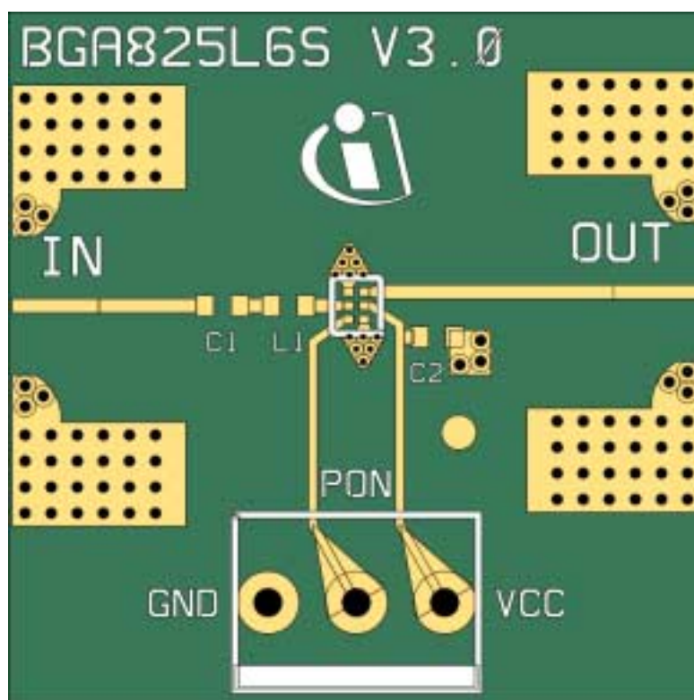
BGA825L6S_Application_Board.vsd
