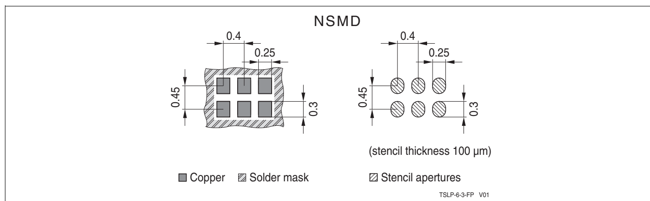
Figure 7 Footprint TSLP-6-3
