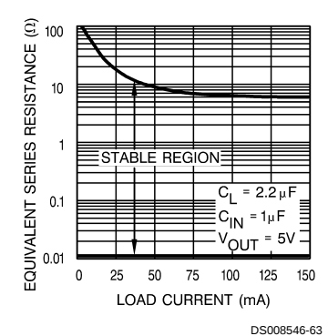
Output Capacitor ESR Range
