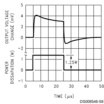
Thermal Response
