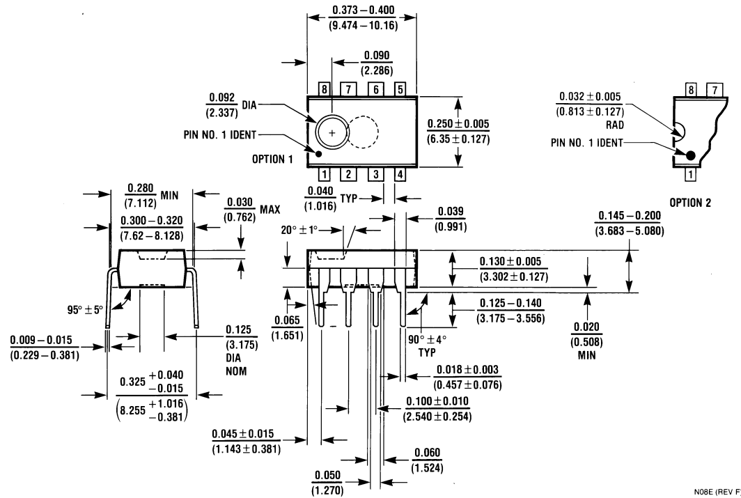
Molded Dual-In-Line Package (N) Order Number LP2951ACN, LP2951CN, LP2951ACN-3.0, LP2951CN-3.0, or LP2951ACN-3.3 or LP2951CN-3.3 NS Package Number NO8E
