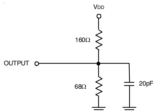
TEST CIRCUIT 1
