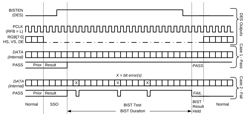
Figure 19. BIST Waveforms
