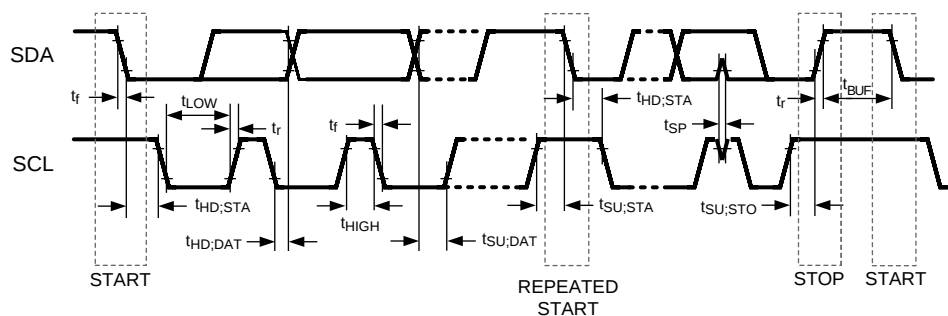
Figure 10. Serial Control Bus Timing Diagram
