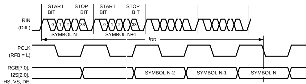
Figure 5. Delay - Latency
