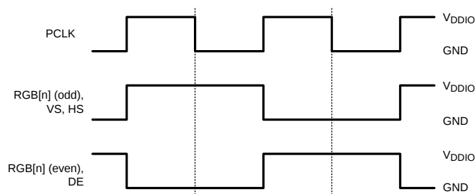
Figure 2. Checker Board Data Pattern
