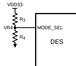
Figure 14. MODE_SEL Connection Diagram
