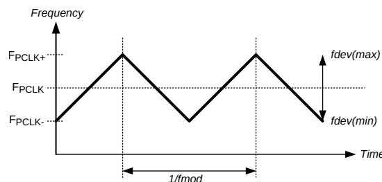
Figure 13. SSCG Waveform
