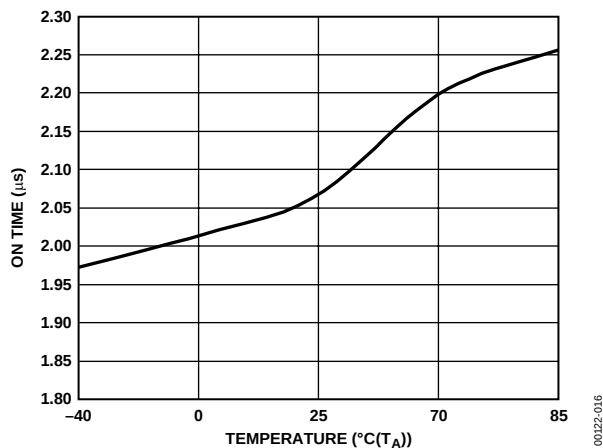
Figure 17. Switch-On Time vs. Temperature
