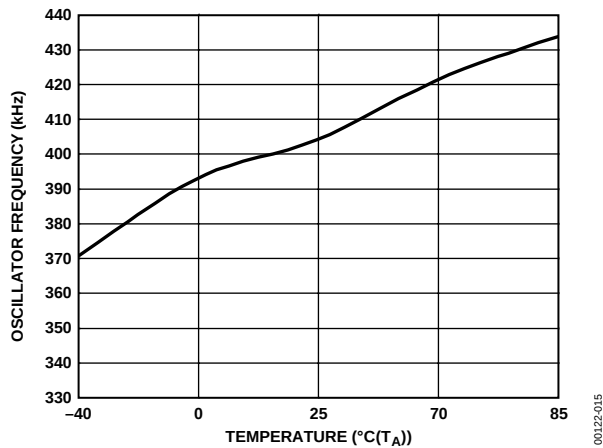
Figure 16. Oscillator Frequency vs. Temperature
