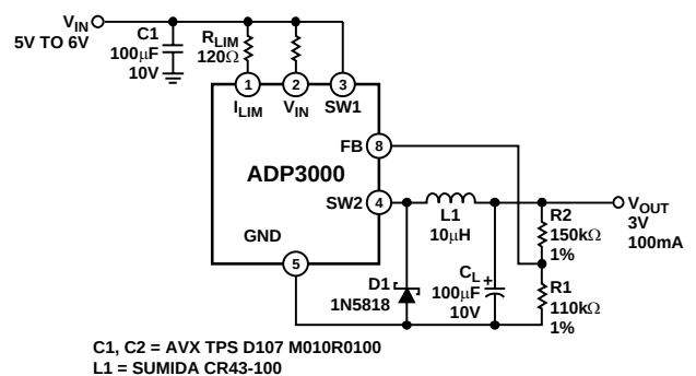
Figure 3. Step-Down Mode Operation
