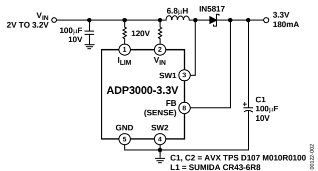
Figure 2. Typical Application
