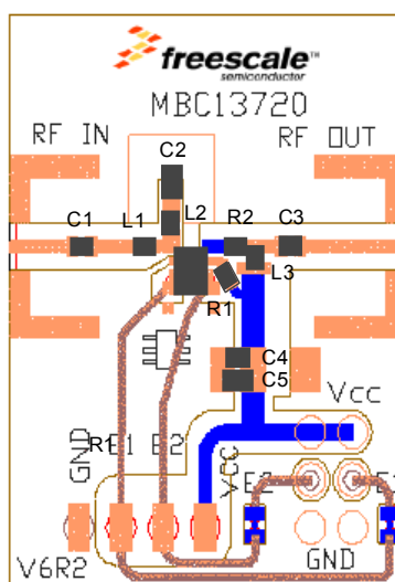
Figure 10. 900 MHz Assembly Diagram
