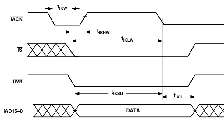
Figure 19. IDMA Write, Long Write Cycle
