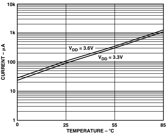
Figure 29. Power-Down Graph
