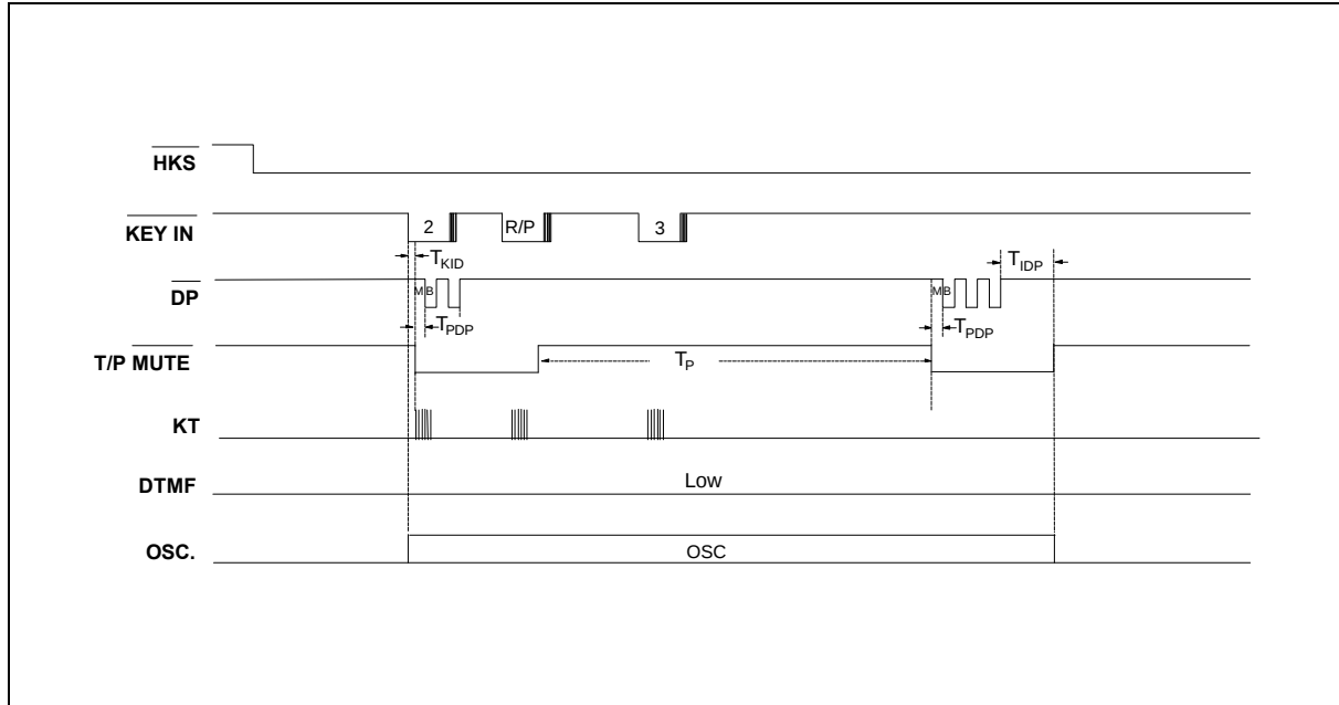
Timing Waveform, continued
