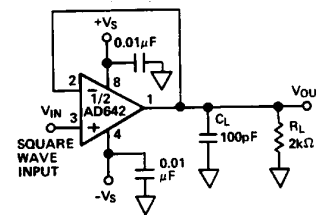
Figure 21c. Unity Gain Follower Pulse Response (Small Signal)
