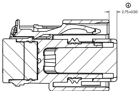
SECTION Z-Z
